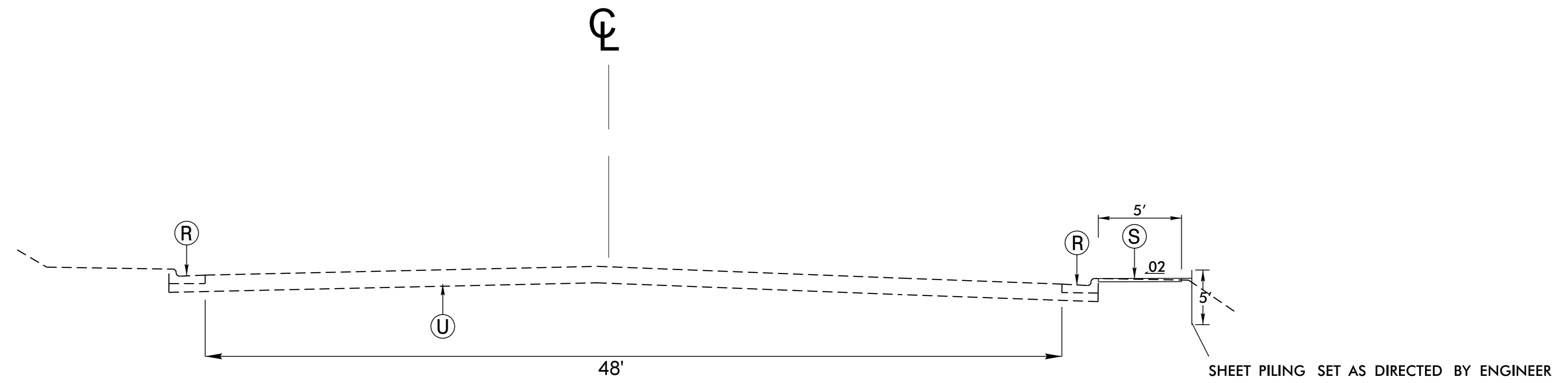
TYPICAL SECTION NO. 1 -L- STA 14+70.00 - 16+98.00
